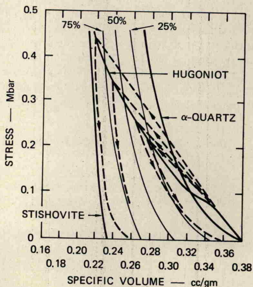
Fig. 4. Stress-volume relief paths in Arkansas novaculite. Loading and relief paths are indicated by the dashed lines.
