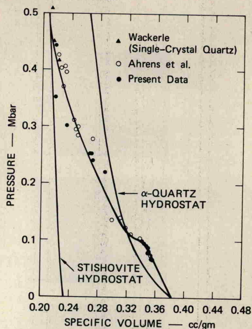
Fig. 3. Pressure-volume Hugoniot for Arkansas novaculite.
